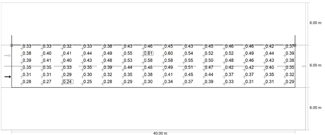
Observer 1: Maintenance value, luminance with dry roadway [ cd/m^2 ] (Iso-illuminance curves)
