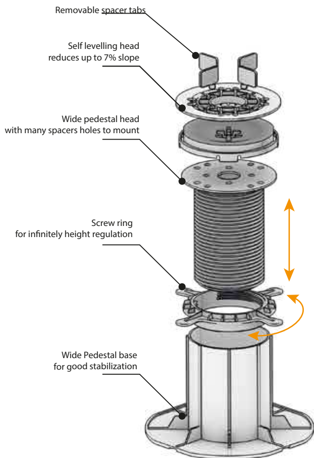
Pedestals elements
