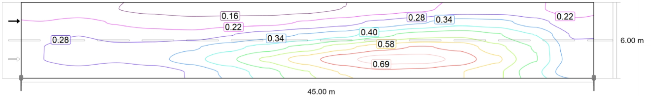
Observer 2: Maintenance value, luminance with dry roadway [ \text{cd}/\text{m}^2 ] (Iso-illuminance curves)
