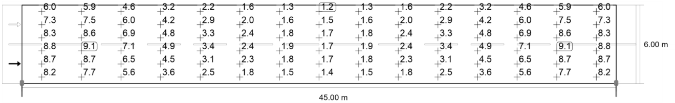
Maintenance value, horizontal illuminance [lx] (Value grid)
