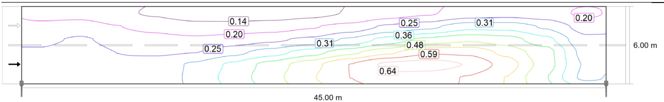
Observer 1: Maintenance value, luminance with dry roadway [cd/m²] (Iso-illuminance curves)
