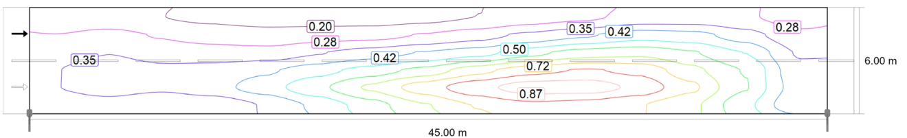
Observer 2: Luminance with new installation [ \text{cd}/\text{m}^2 ] (Iso-illuminance curves)
