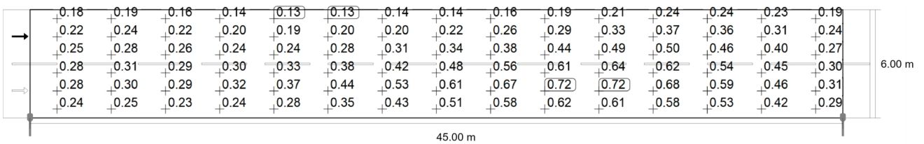
Observer 2: Maintenance value, luminance with dry roadway [ \text{cd}/\text{m}^2 ] (Value grid)
