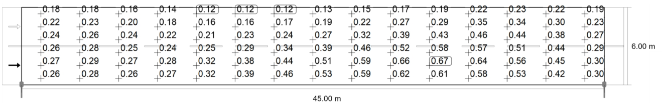
Observer 1: Maintenance value, luminance with dry roadway [cd/m²] (Value grid)
