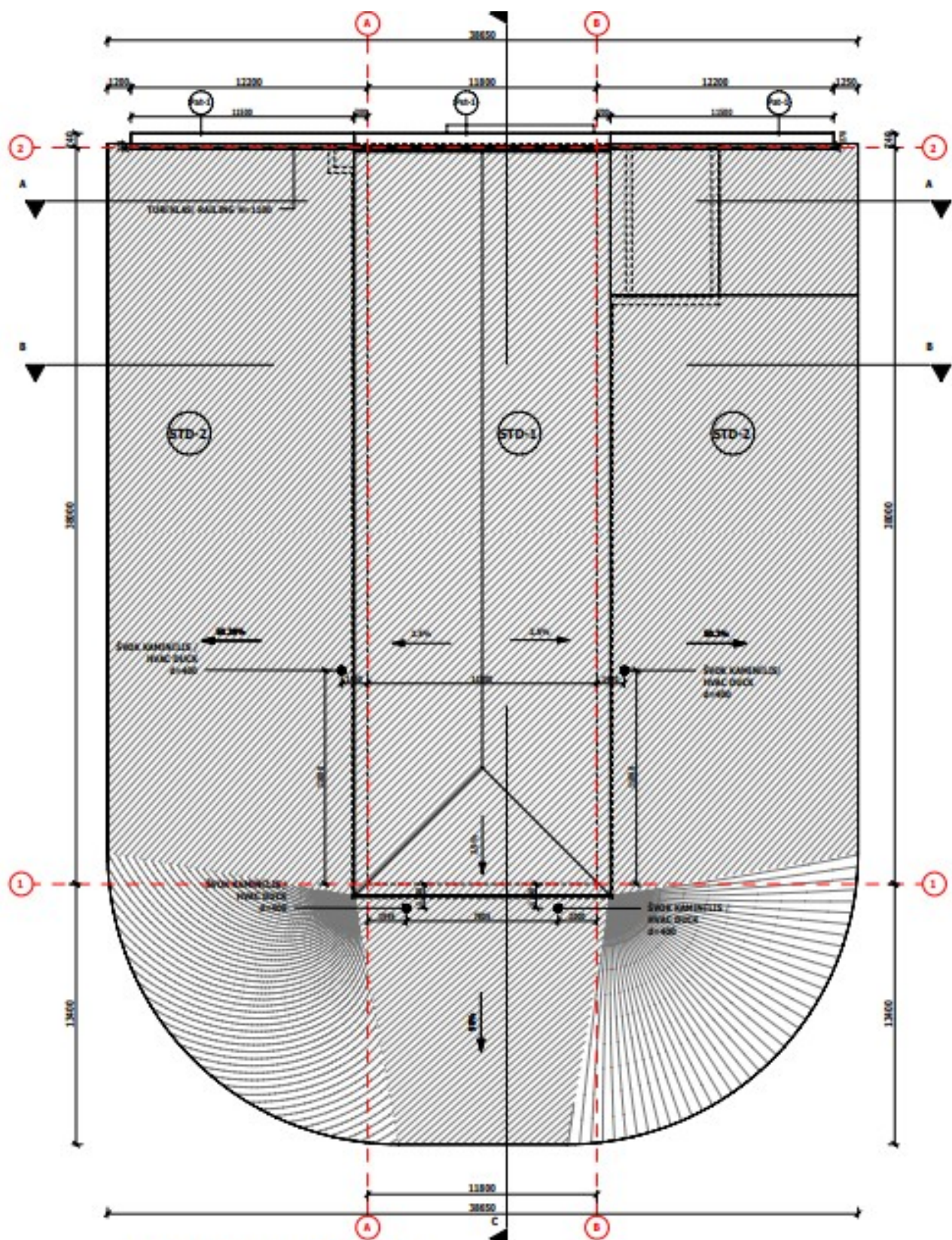
STOGO PLANAS/ ROOF PLAN 1 : 200
