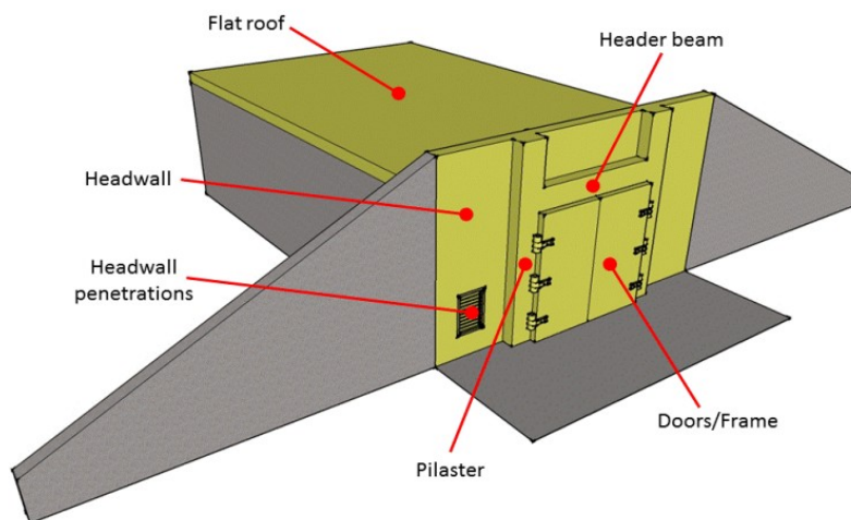
Figure 2-2: Typical ECM Blast Resisting Elements
