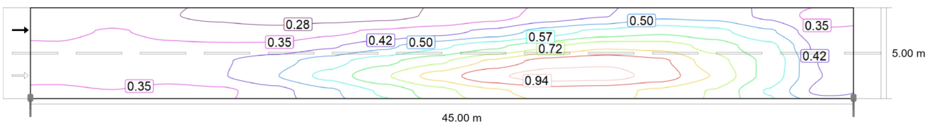
Observer 2: Luminance with new installation [ \text{cd}/\text{m}^2 ] (Iso-illuminance curves)
