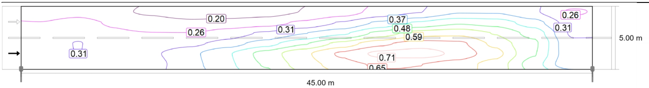
Observer 1: Maintenance value, luminance with dry roadway [ cd/m^2 ] (Iso-illuminance curves)
