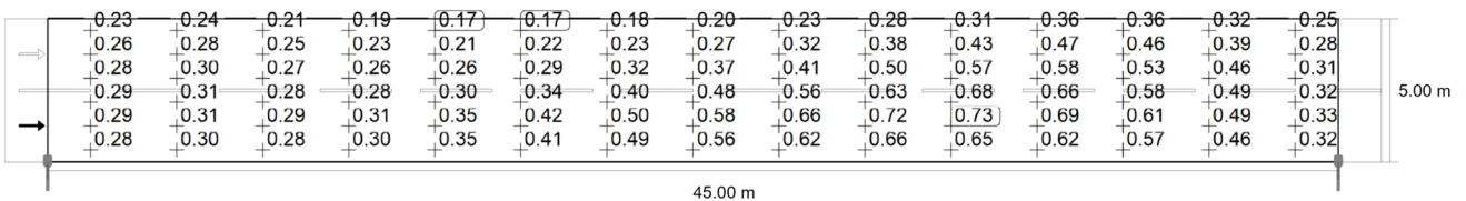
Observer 1: Maintenance value, luminance with dry roadway [ cd/m^2 ] (Value grid)
