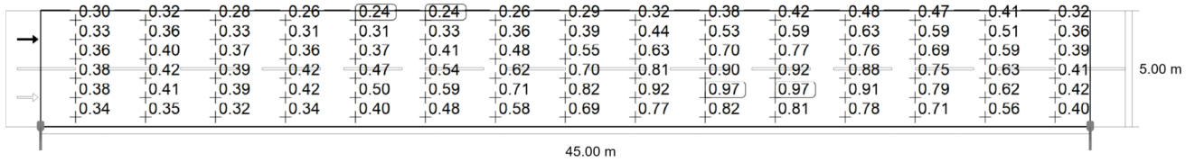
Observer 2: Luminance with new installation [cd/m 2 ] (Value grid)
