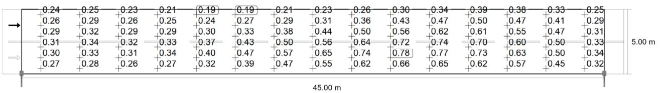
Observer 2: Maintenance value, luminance with dry roadway [ \text{cd}/\text{m}^2 ] (Value grid)
