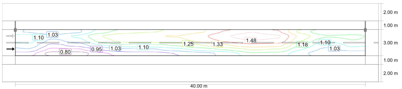
Observer 1: Luminance with new installation [ \text{cd/m}^2 ] (Iso-illuminance curves)
