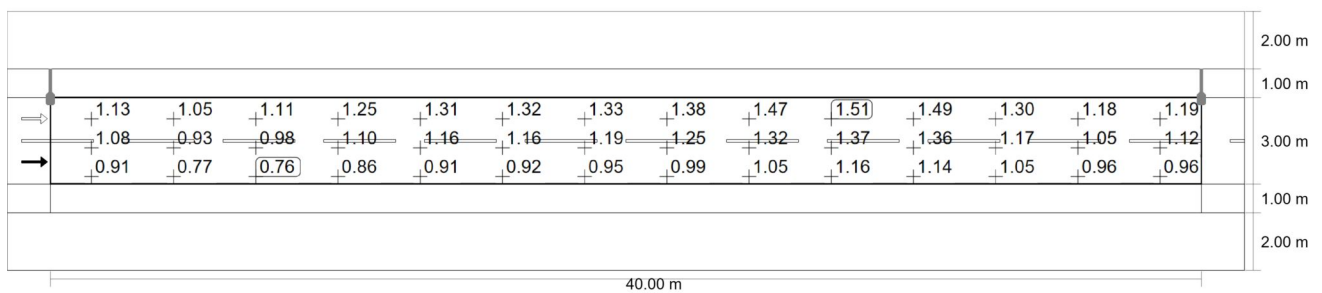
Observer 1: Luminance with new installation [ \text{cd/m}^2 ] (Value grid)
