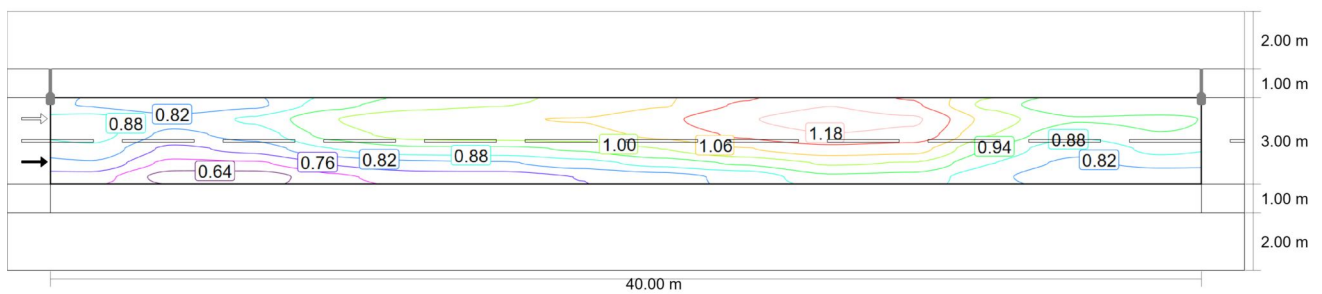
Observer 1: Maintenance value, luminance with dry roadway [ \text{cd/m}^2 ] (Iso-illuminance curves)
