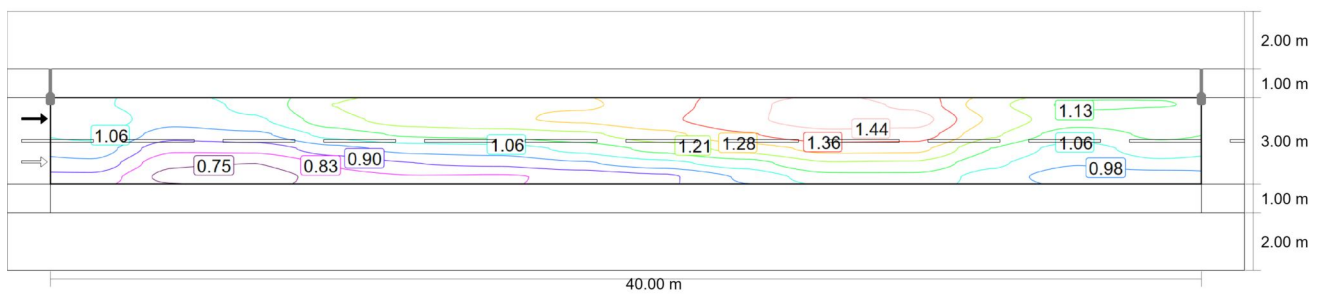
Observer 2: Luminance with new installation [ \text{cd/m}^2 ] (Iso-illuminance curves)
