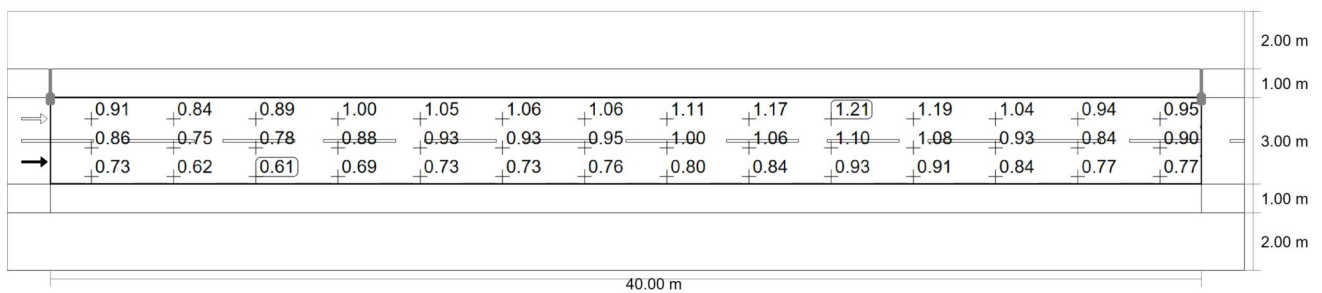
Observer 1: Maintenance value, luminance with dry roadway [ \text{cd/m}^2 ] (Value grid)
