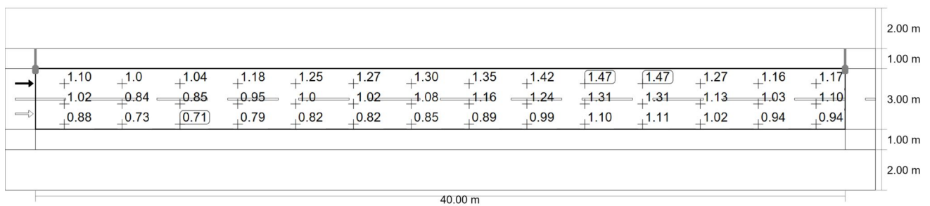
Observer 2: Luminance with new installation [ \text{cd/m}^2 ] (Value grid)
