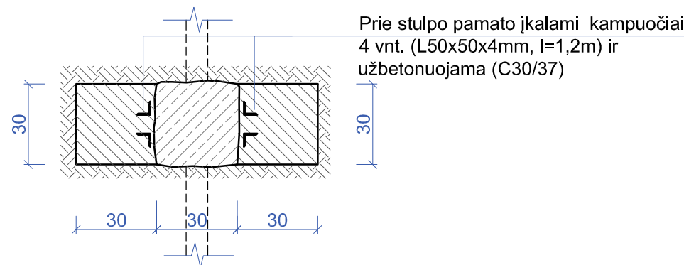
3-3 M 1:20
