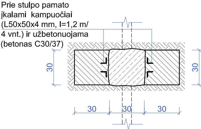
3-3 M 1:20
